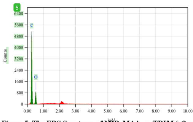
Figure 5. The EDS Spectrum of MIP_MAA-co-TRIM (after washed)
