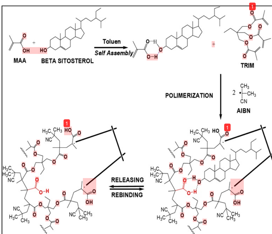
Figure 2. Proposed schemes for MIP_MAA-co-TRIM synthesis pathway
