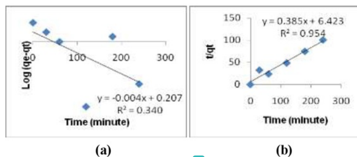
Figure 10. The Kinetic curves of (a) pseudo-order first and (b) pseudo-order second for \beta -sitosterol adsorption by MIP_MAA-co-TRIM
