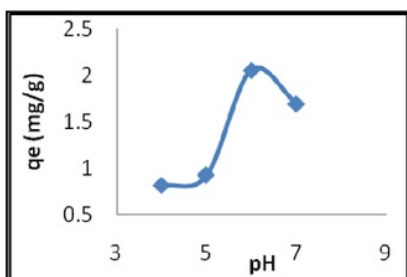
Figure 8. The pH optimum curve of MIP_MAA-co-TRIM
