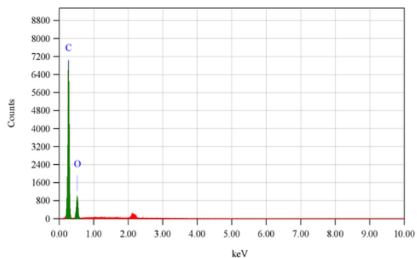
Figure 4. The EDS Spectrum of MIP_MAA-co-TRIM (before washing)
